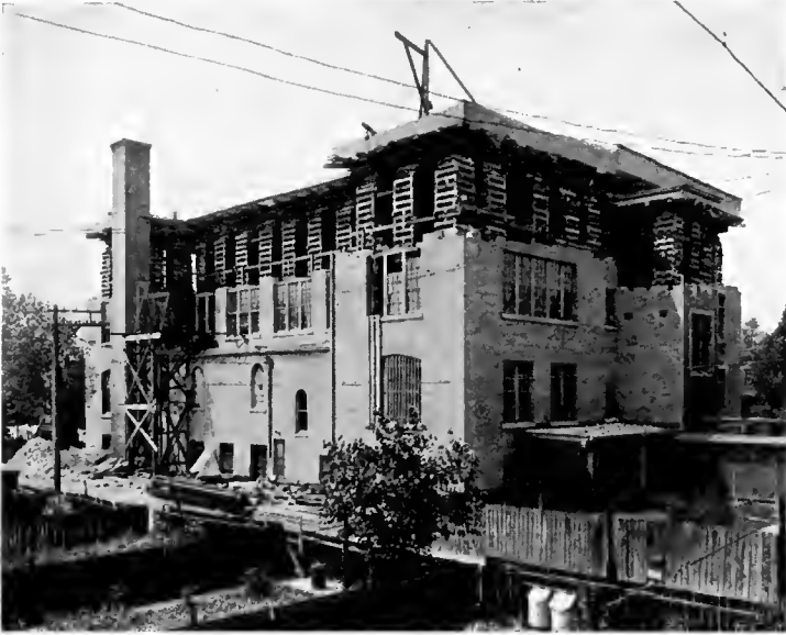
RAISING AND SHORING A FIREPROOF SCHOOL HOUSE
